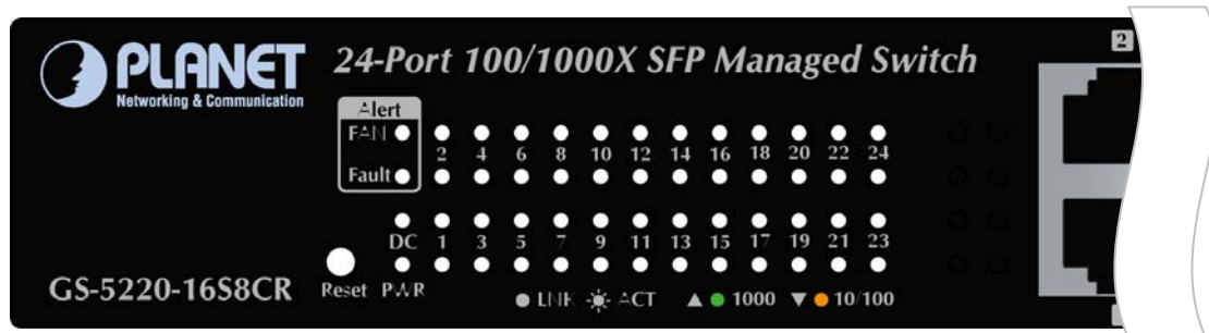
Figure 2-1-9: GS-5220-16S8CR LED on Front Panel
