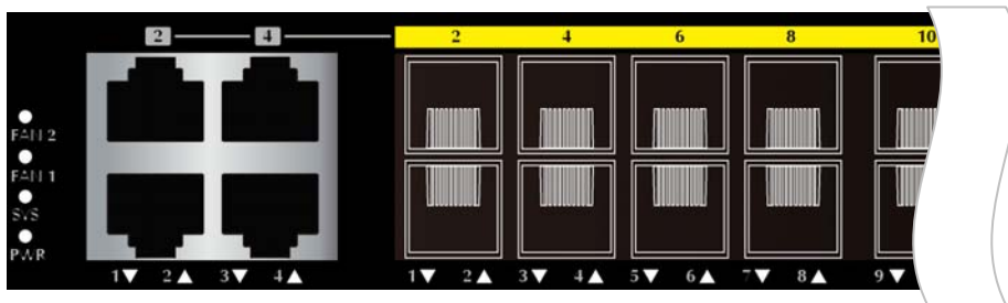
Figure 2-1-10: Front Panel LEDs of GS-5220-44S4C
