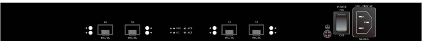
Figure 2-1-17: Rear Panel of GS-5220-46S2C4X
